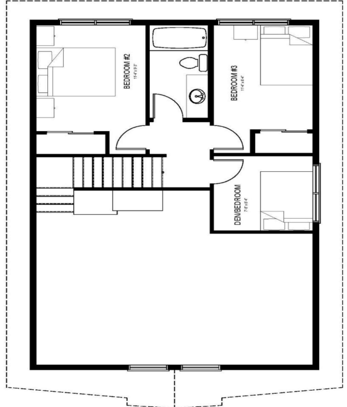
THE PALO | 36'4" X 24'4" | 1320 sq.ft. | 3 Bedroom s + Den | 2 Bathroom s |
