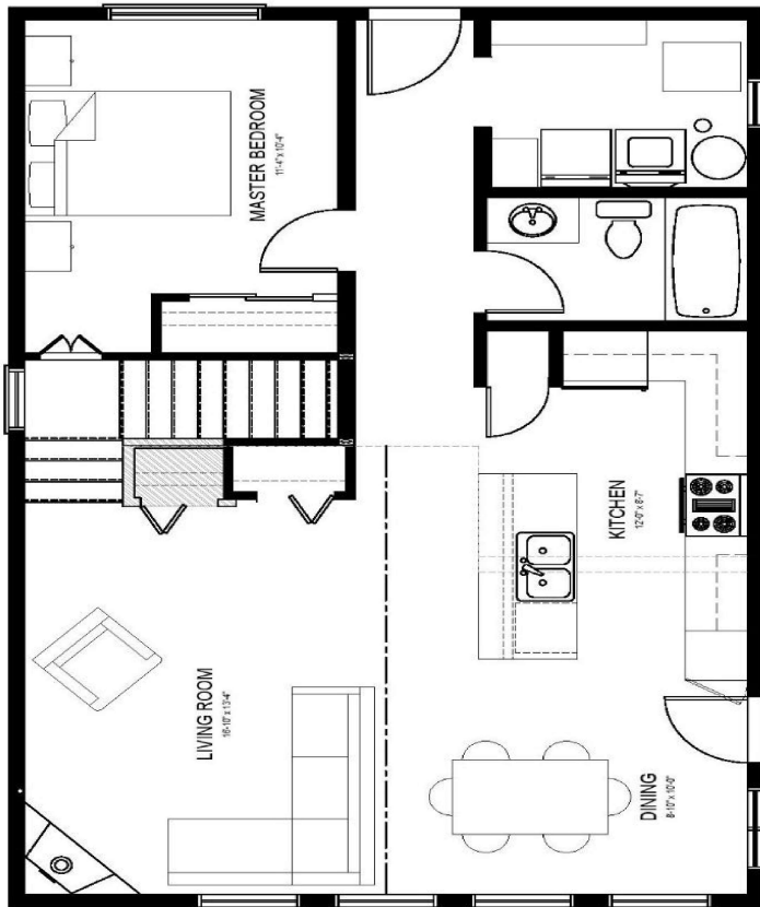
THE PALO | 36'4" X 24'4" | 1320 sq.ft. | 3 Bedroom s + Den | 2 Bathroom s |
