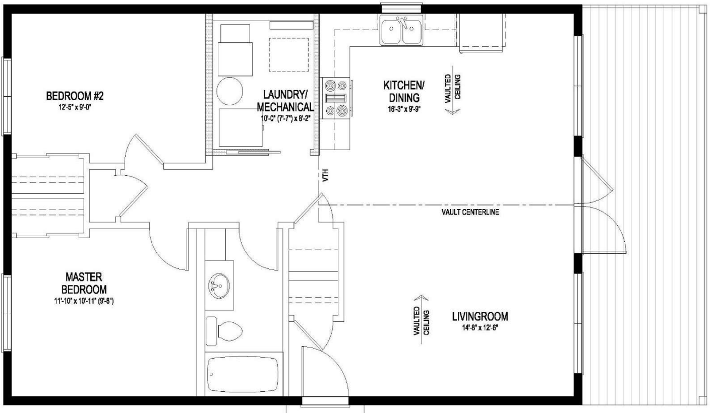
THE HARPTREE I | 37' X 24' | 888 sq.ft. | 2 Bedroom s | 1 Bathroom |
