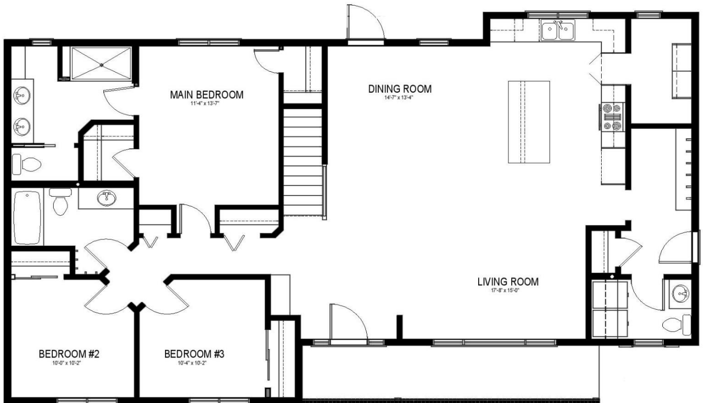
THE VANGUARD | 56' X 33' 4" | 1616 sq.ft. | 3 Bedroom s | 3 Bathroom s |
